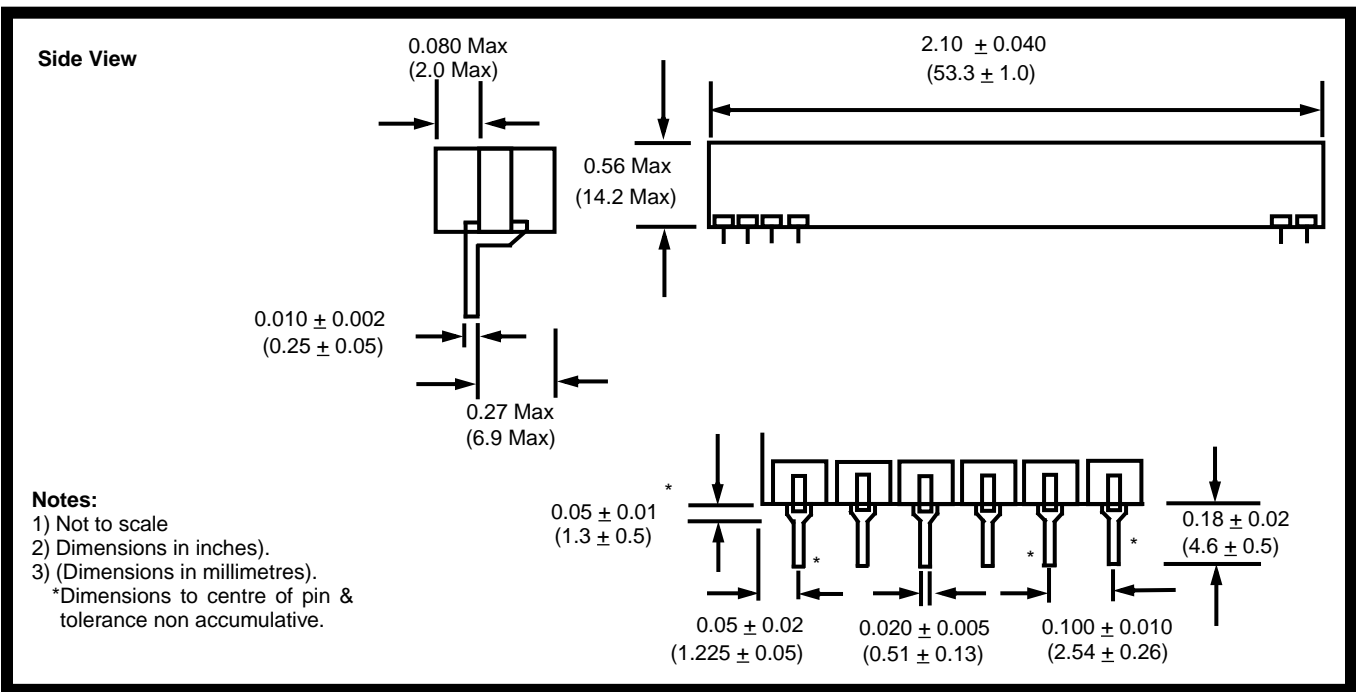
Figure 3 - Mechanical Data
